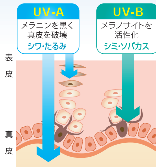
Squalane
